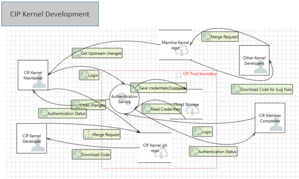
Figure 2: CIP Kernel Development DFD
