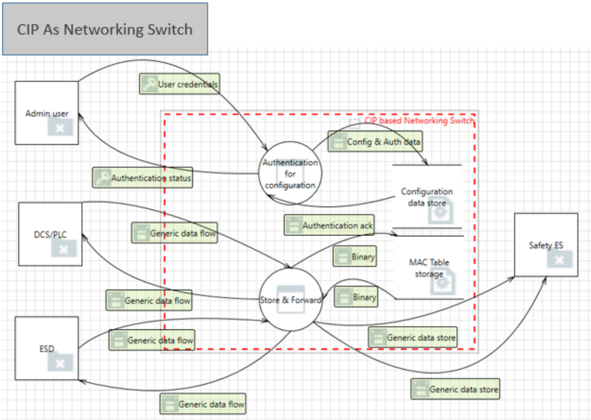
Figure 5: CIP As Networking Use Case DFD
